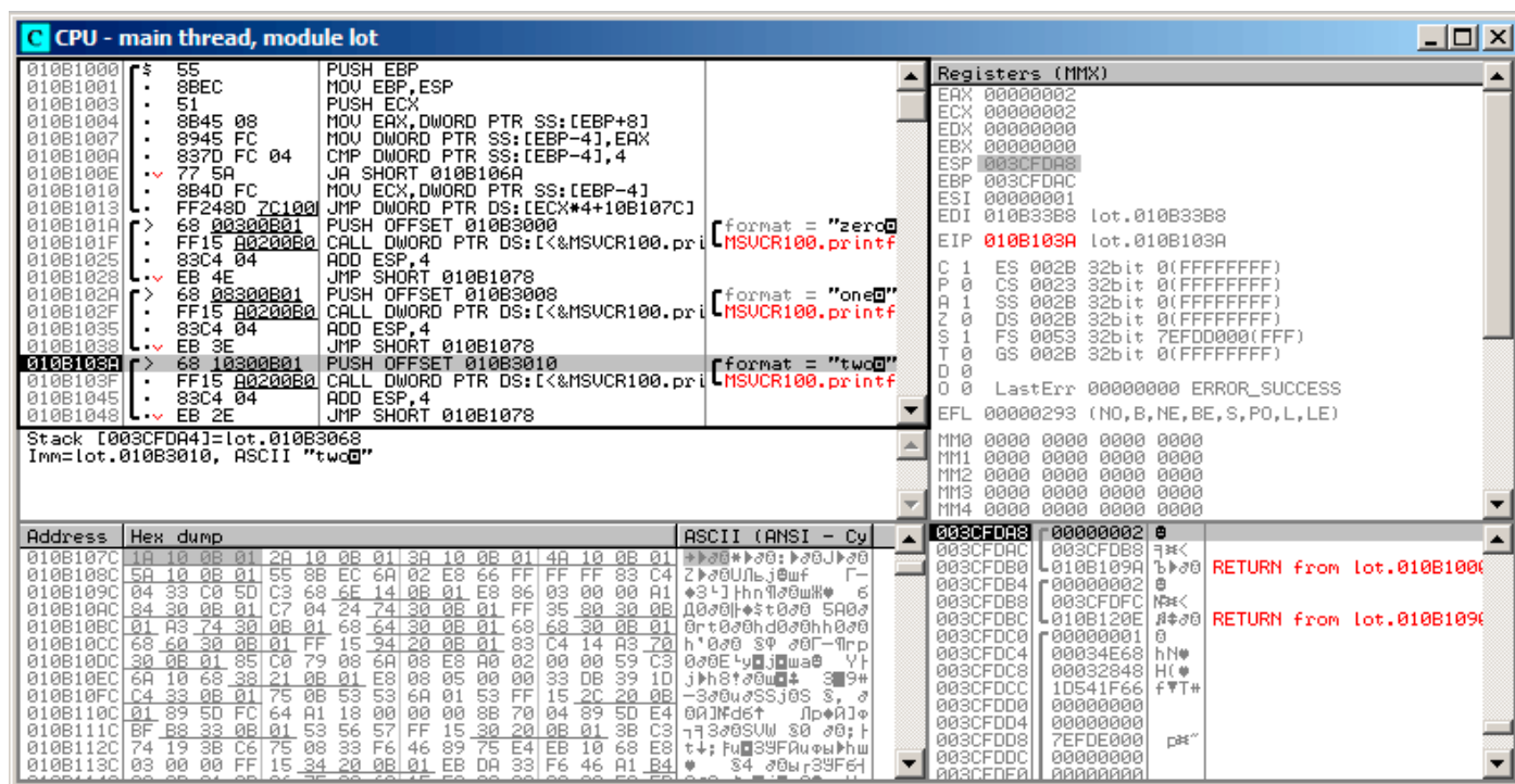
Figure 1.53: OllyDbg: now we at the case: label
