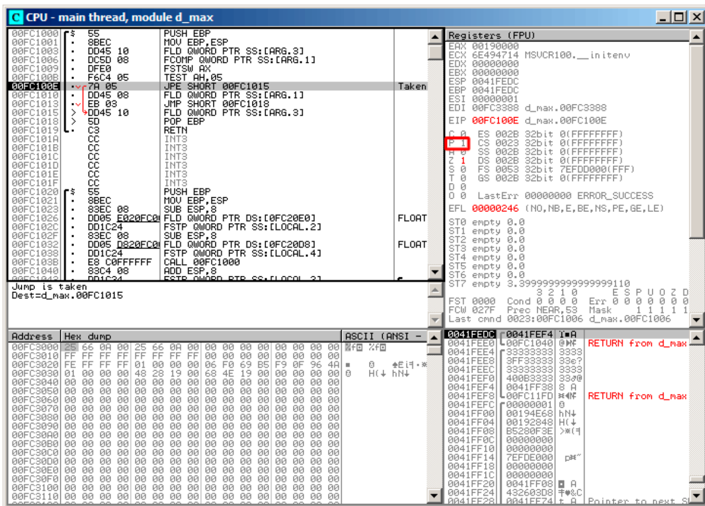
Figure 1.70: OllyDbg: TEST has been executed
