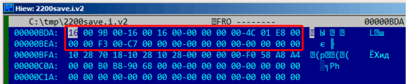
Figure 9.15: Hiew: state 1
