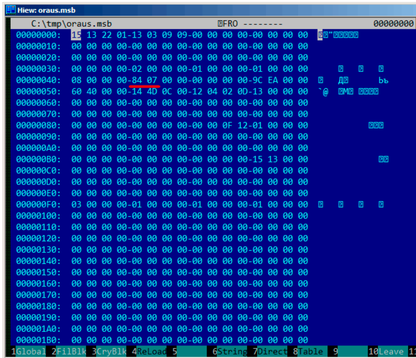
Figure 9.28: Hiew: file header
