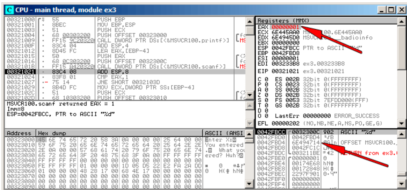
Figure 1.20: OllyDbg: scanf() returning error
