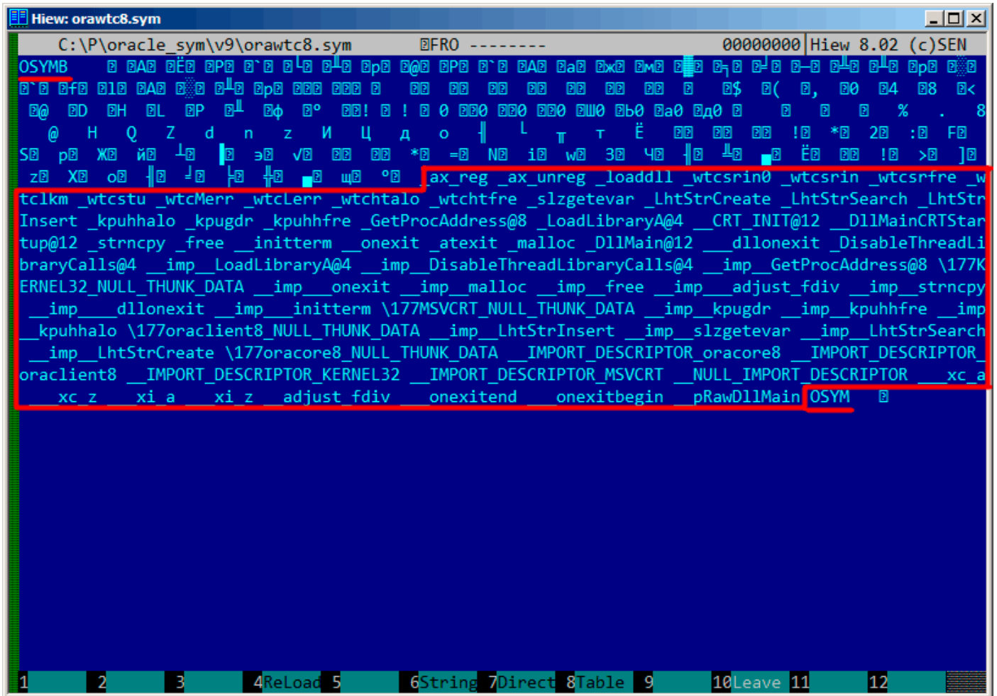
Figure 9.22: OSYM signature and text strings
