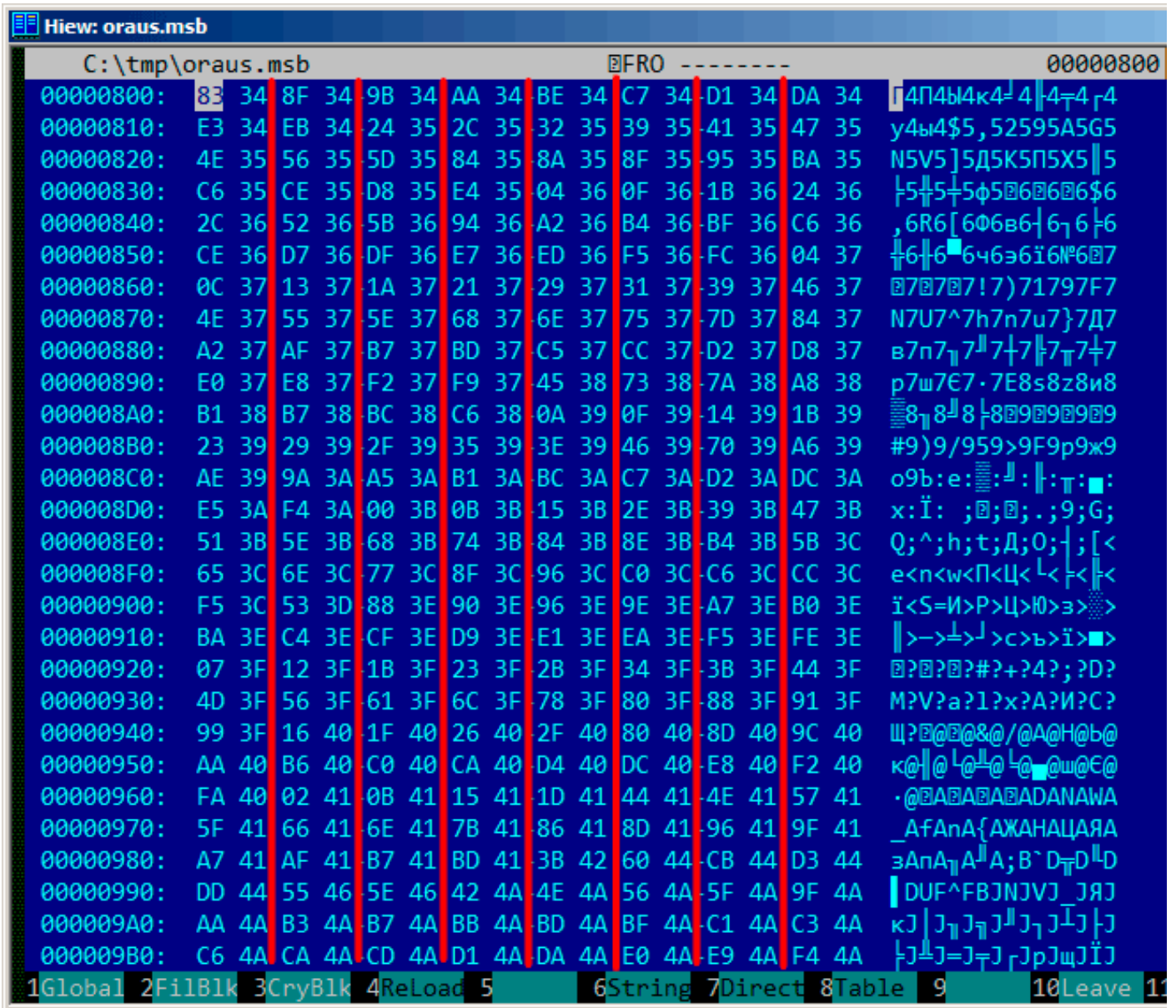
Figure 9.29: Hiew: last_errnos table
