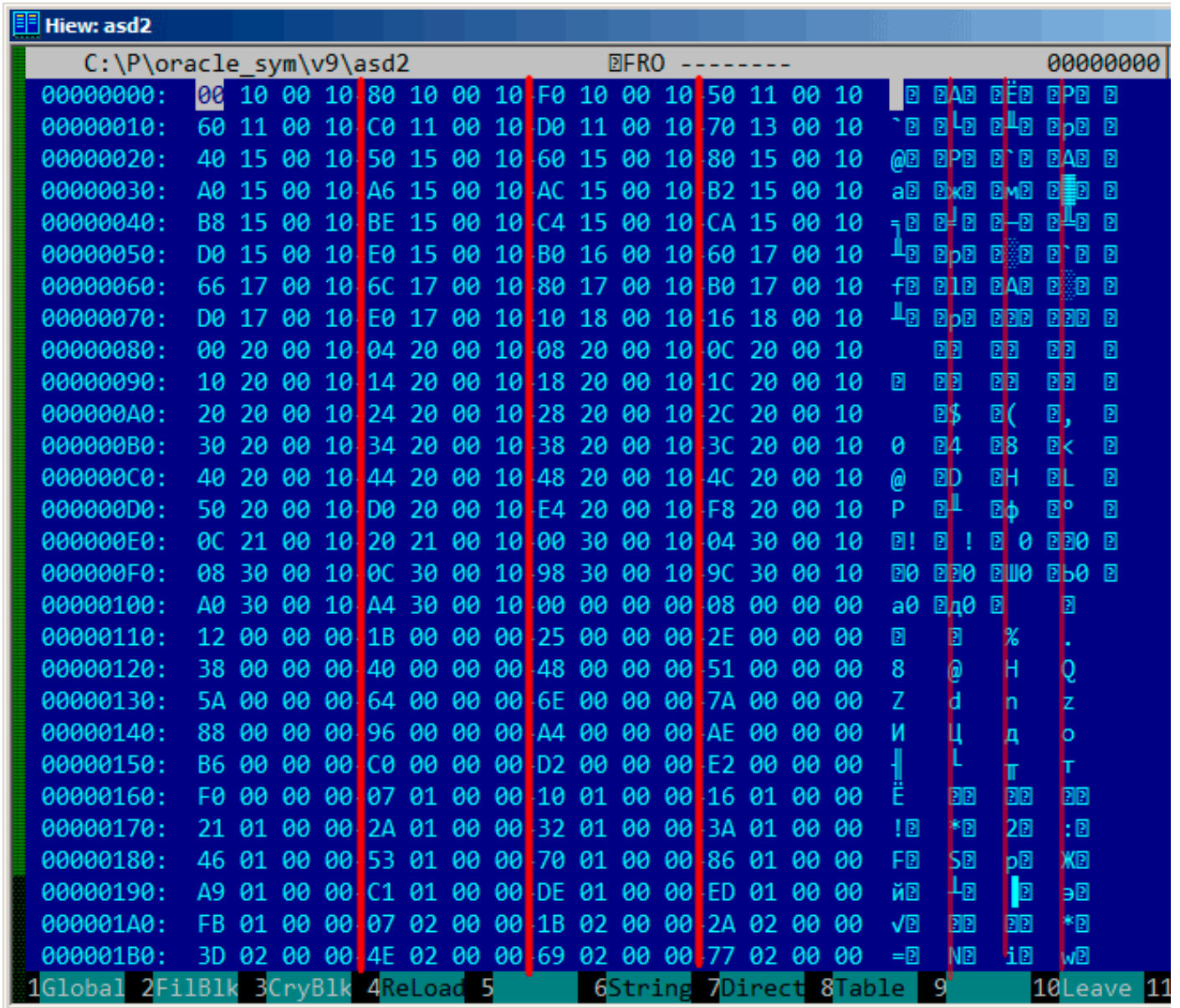
Figure 9.24: Binary block patterns
