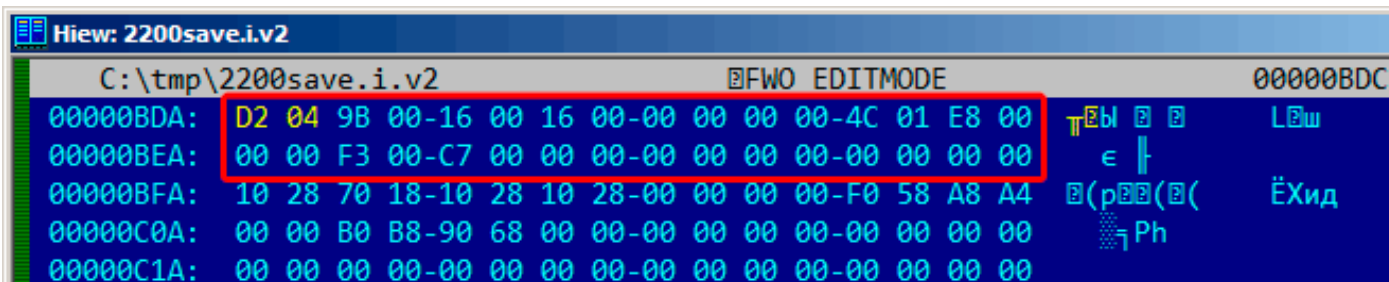
Figure 9.16: Hiew: let's write 1234 (0x4D2) there
