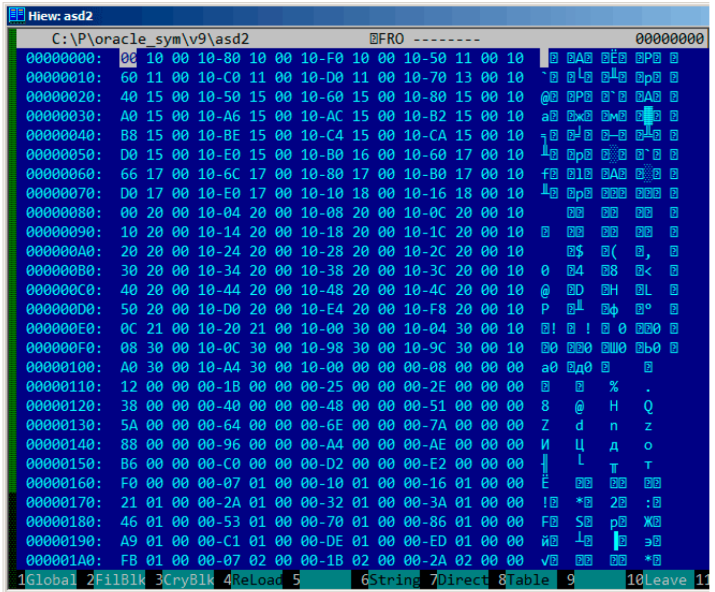
Figure 9.23: Binary block
