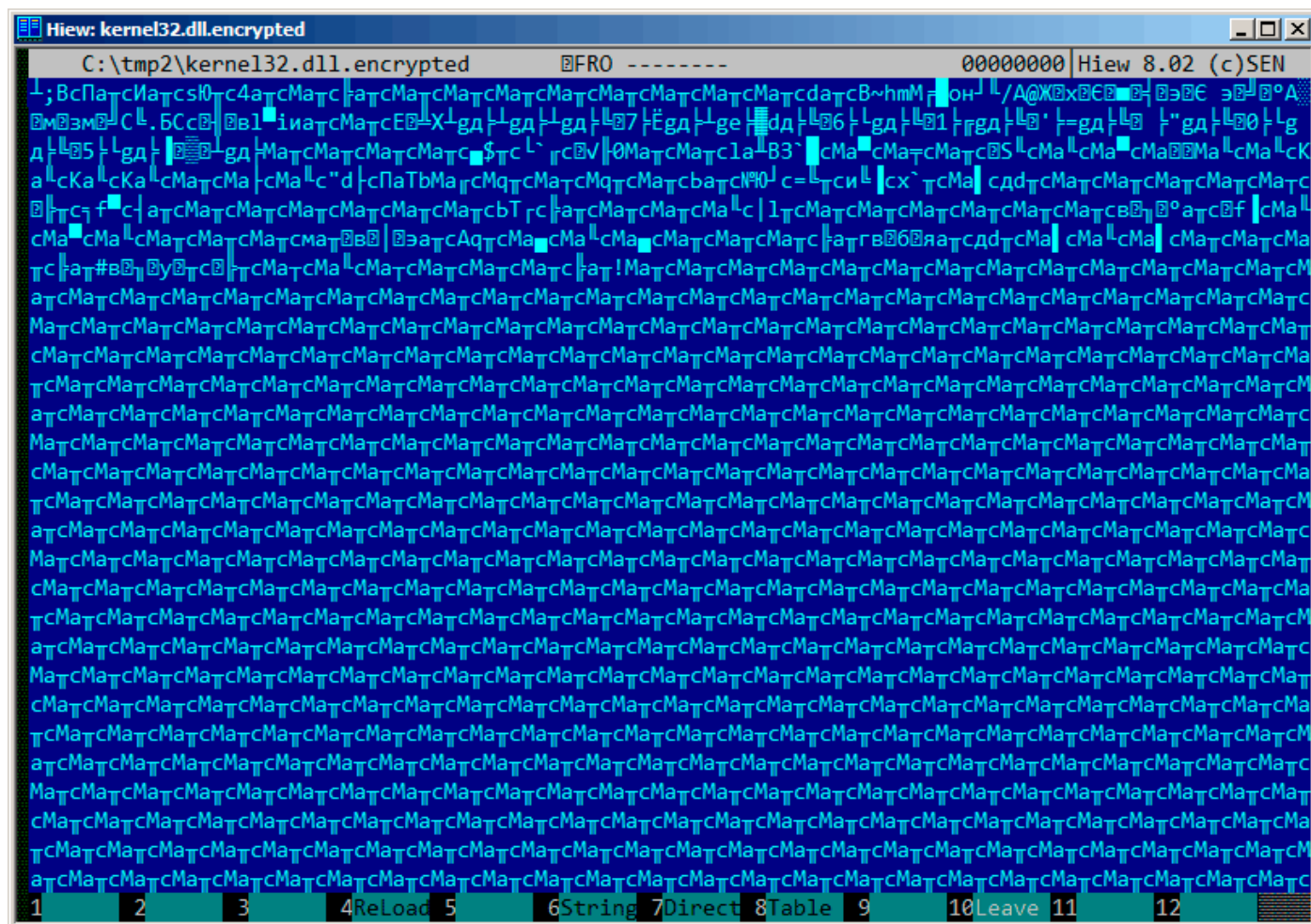
Figure 9.4: “Encrypted” file
