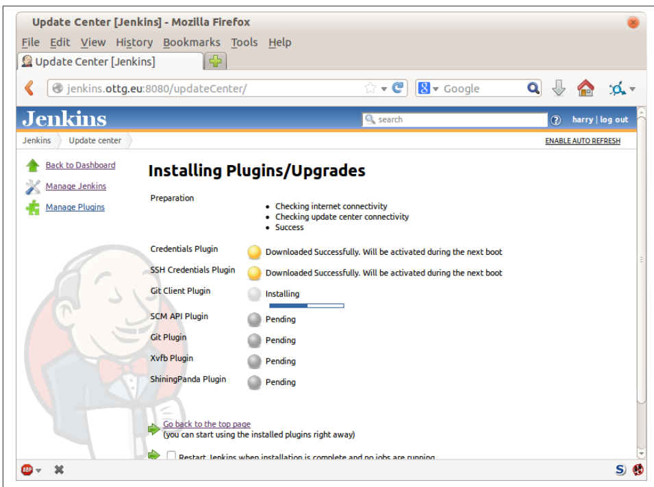
Figure 20-3. Installing plugins...
