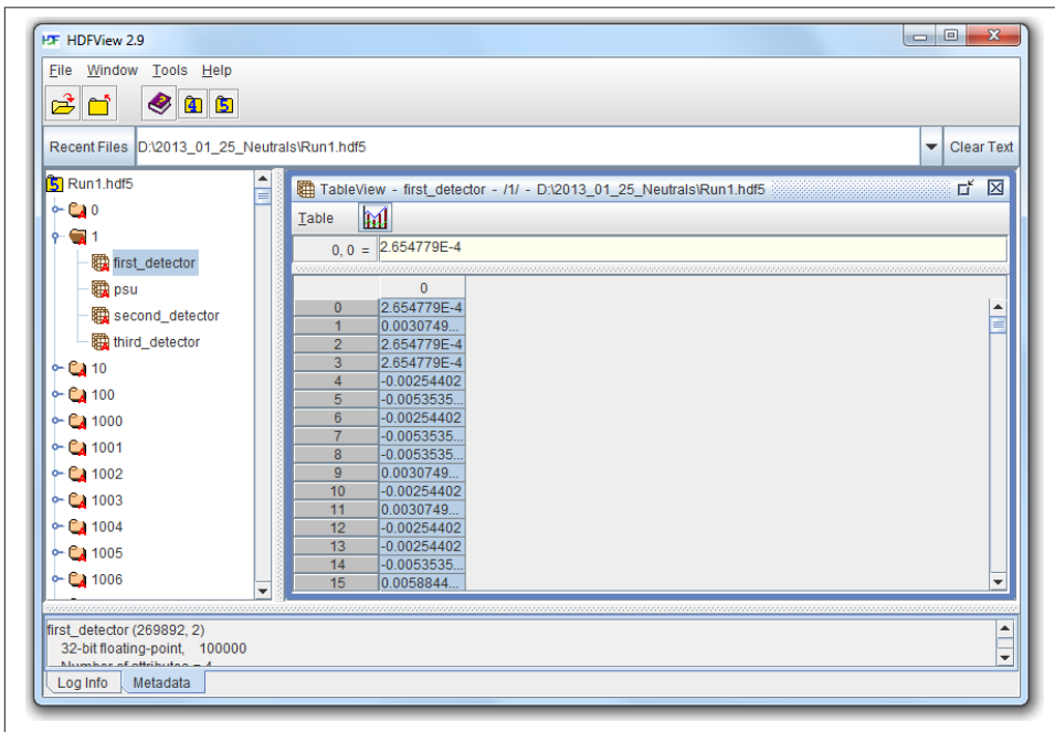
Figure 2-2. HDFView
