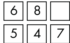
Figure 1-6: A particular starting configuration for a reduced, 2x3 sliding tile puzzle
