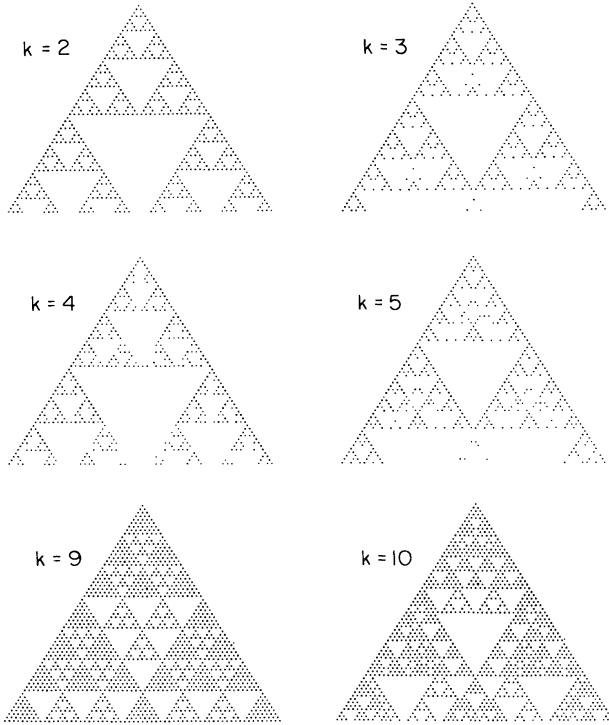
FIG. 29. Patterns generated by evolution of one-dimensional cellular automata with k states per site according to a modulo- k rule, starting from an initial configuration containing a single nonzero site with value one. At each time step, the value of a site is the sum of the values of its two nearest neighbors at the previous time step. Configurations obtained at successive time steps are shown on successive lines. Sites with value zero are indicated as blanks; *, +, and - represent, respectively, values one, two, and three, and in the lower two patterns, \rho represents any nonzero value. In the large time limit, all the patterns tend to a self-similar form, with definite fractal dimensions.
